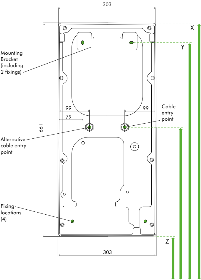
REAR ELEVATION
