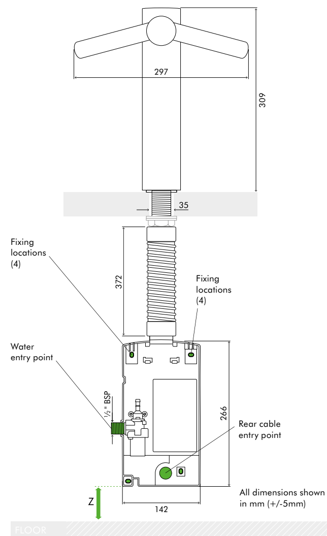
REAR ELEVATION
