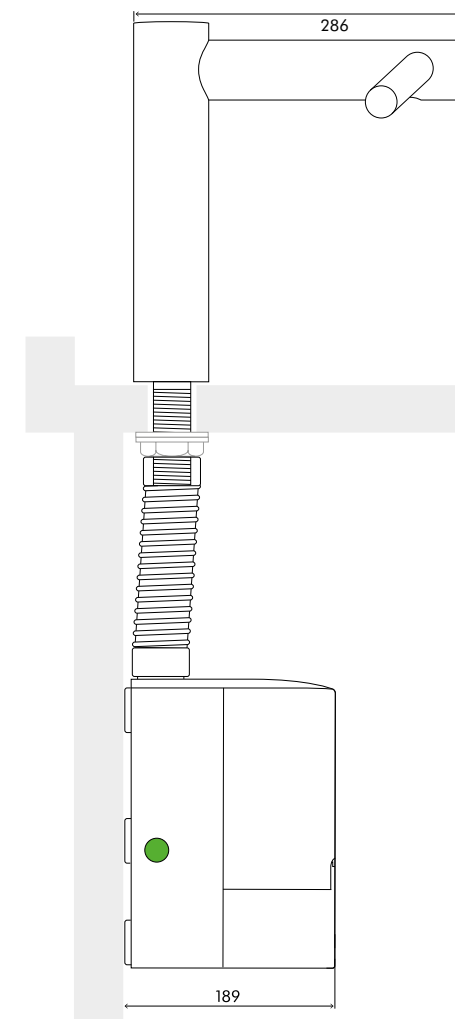
SIDE ELEVATION
